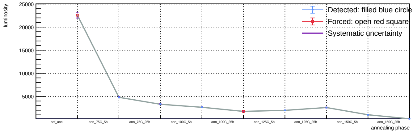
Sensor B1, T = 20\text{ C} , v_{\text{over}} = 5\text{ V} - Spot 65: luminosity vs phase
