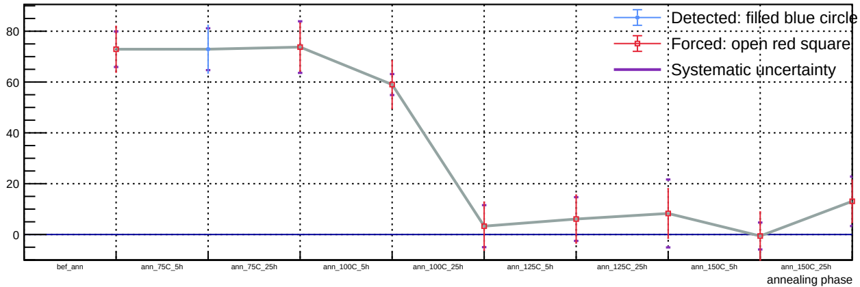
Sensor B1, T = 20\text{ C} , v_{\text{over}} = 5\text{ V} - Spot 66: luminosity vs phase
