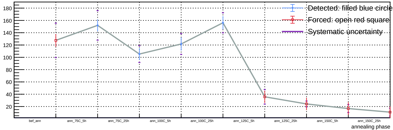
Sensor B1, T = 20\text{ C} , v_{\text{over}} = 5\text{ V} - Spot 67: luminosity vs phase
