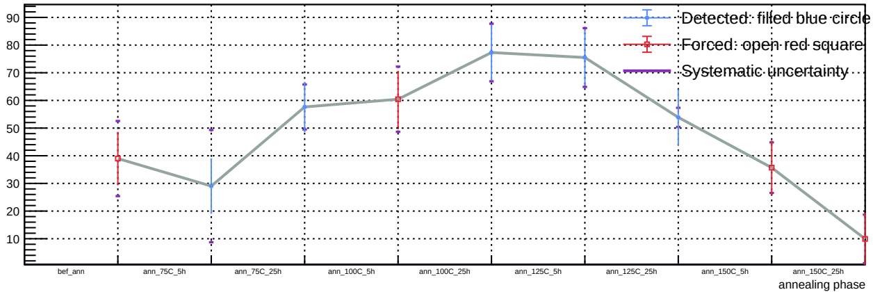
Sensor B1, T = 20\text{ C} , v_{\text{over}} = 5\text{ V} - Spot 68: luminosity vs phase
