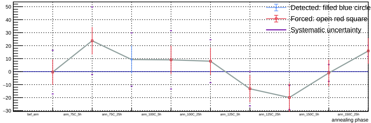
Sensor B1, T = 20\text{ C} , v_{\text{over}} = 5\text{ V} - Spot 69: luminosity vs phase
