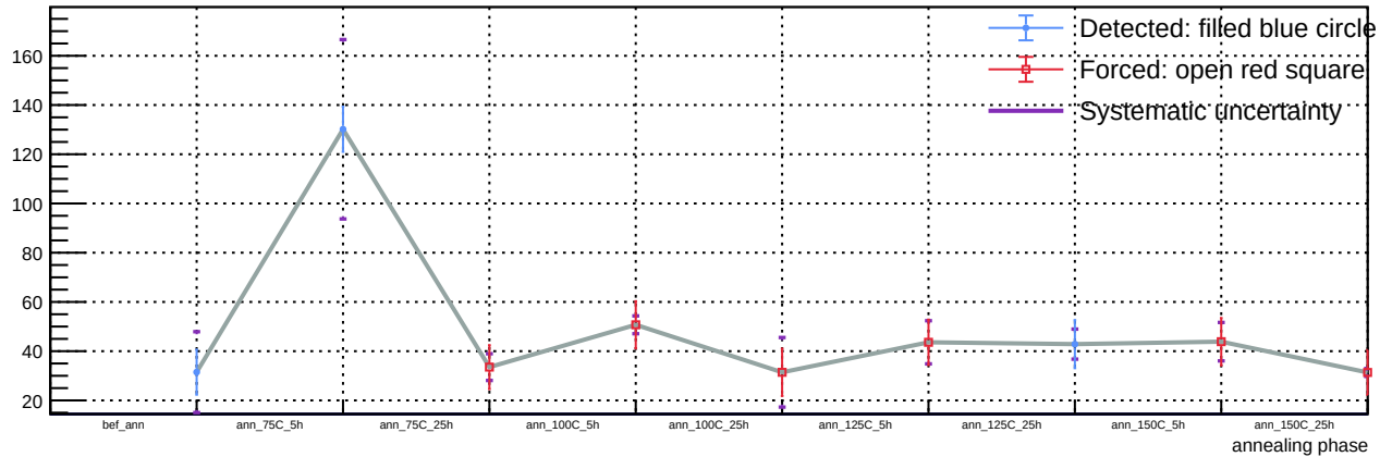
Sensor B1, T = 20\text{ C} , v_{\text{over}} = 5\text{ V} - Spot 7: luminosity vs phase
