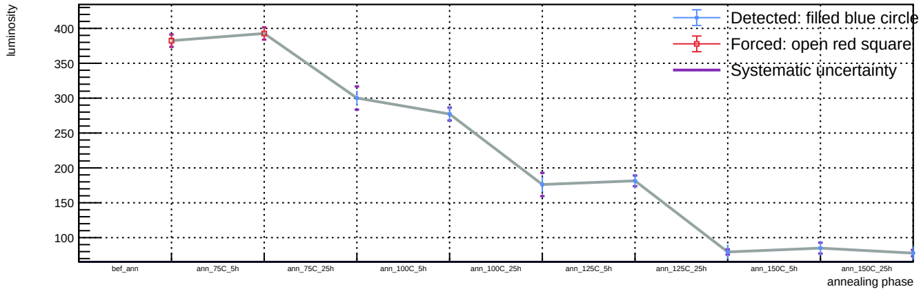
Sensor B1, T = 20\text{ C} , v_{\text{over}} = 5\text{ V} - Spot 74: luminosity vs phase
