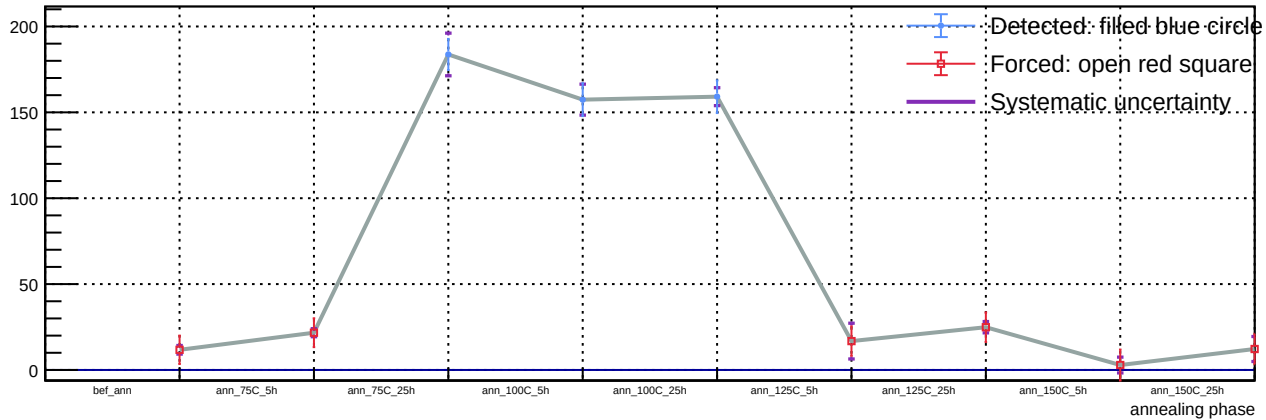
Sensor B1, T = 20\text{ C} , v_{\text{over}} = 5\text{ V} - Spot 76: luminosity vs phase
