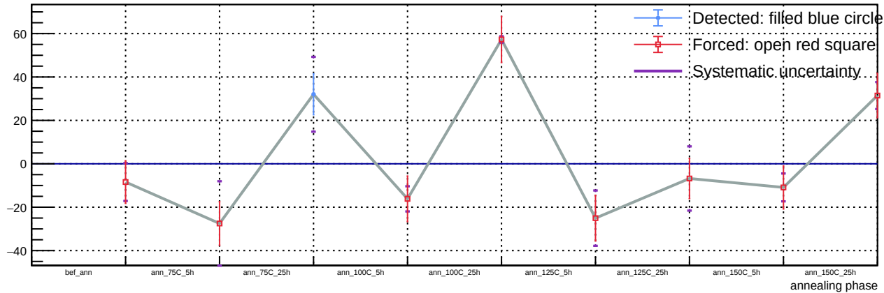
Sensor B1, T = 20\text{ C} , v_{\text{over}} = 5\text{ V} - Spot 79: luminosity vs phase
