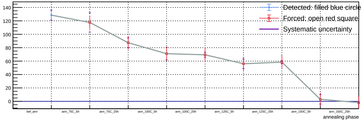
Sensor B1, T = 20\text{ C} , v_{\text{over}} = 5\text{ V} - Spot 8: luminosity vs phase
