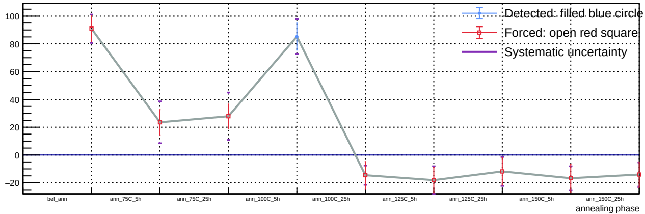
Sensor B1, T = 20\text{ C} , v_{\text{over}} = 5\text{ V} - Spot 81: luminosity vs phase
