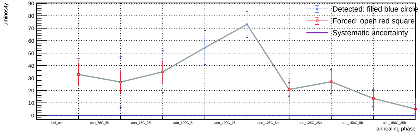
Sensor B1, T = 20\text{ C} , v_{\text{over}} = 5\text{ V} - Spot 82: luminosity vs phase
