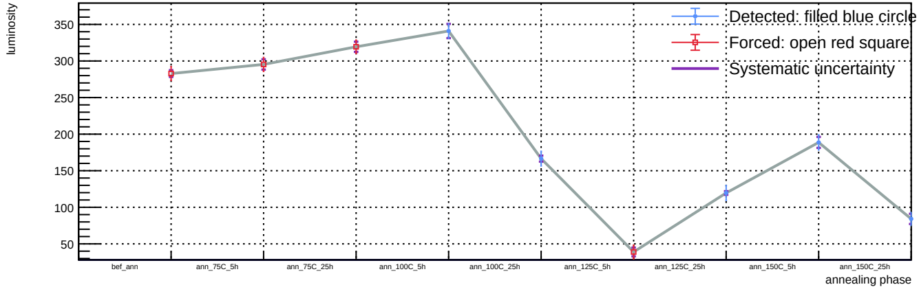
Sensor B1, T = 20\text{ C} , v_{\text{over}} = 5\text{ V} - Spot 83: luminosity vs phase
