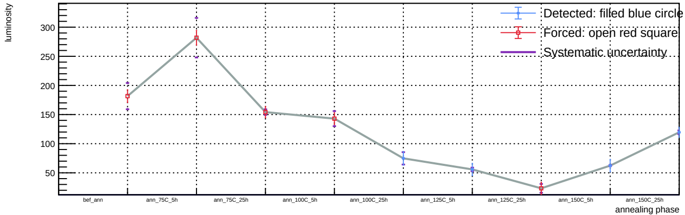
Sensor B1, T = 20\text{ C} , v_{\text{over}} = 5\text{ V} - Spot 88: luminosity vs phase
