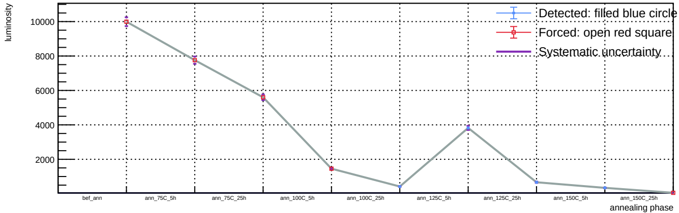
Sensor B1, T = 20\text{ C} , v_{\text{over}} = 5\text{ V} - Spot 89: luminosity vs phase
