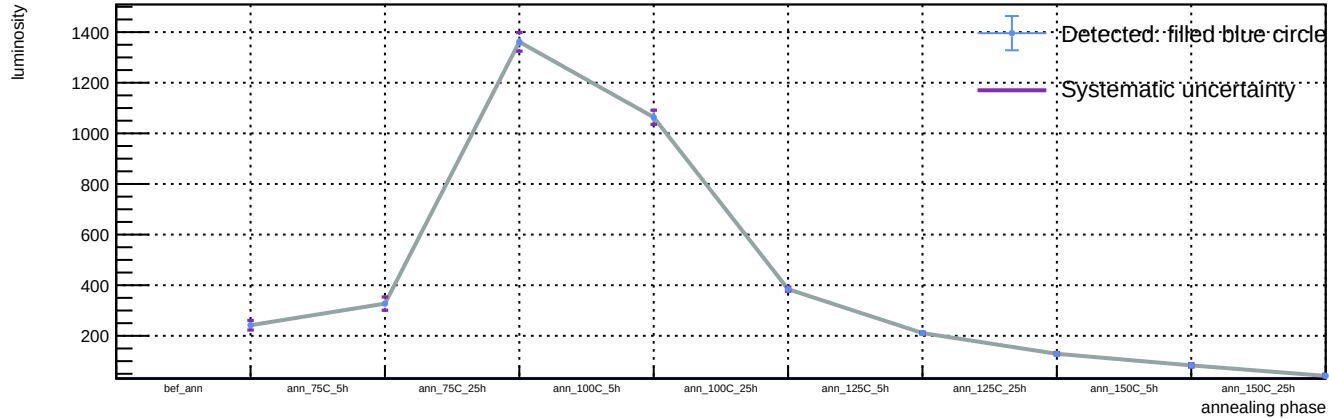
Sensor B1, T = 20\text{ C} , v_{\text{over}} = 5\text{ V} - Spot 9: luminosity vs phase
