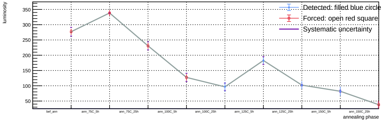
Sensor B1, T = 20\text{ C} , v_{\text{over}} = 5\text{ V} - Spot 92: luminosity vs phase
