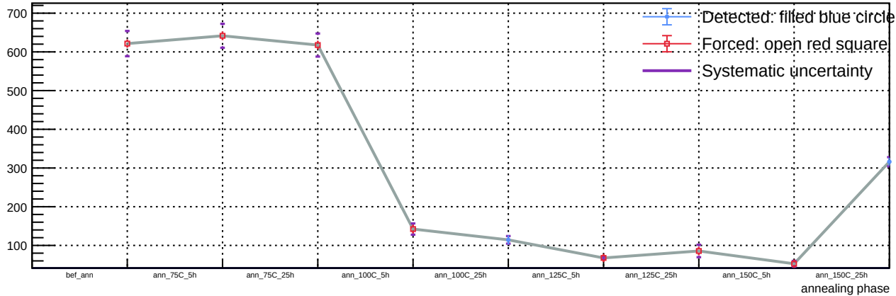
Sensor B1, T = 20\text{ C} , v_{\text{over}} = 5\text{ V} - Spot 93: luminosity vs phase
