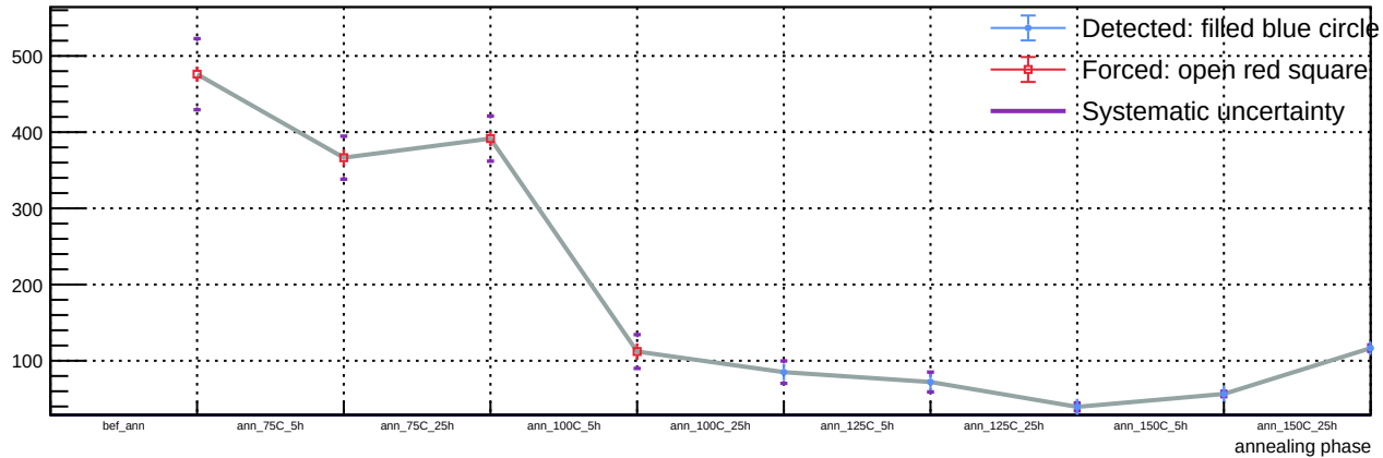
Sensor B1, T = 20\text{ C} , v_{\text{over}} = 5\text{ V} - Spot 94: luminosity vs phase
