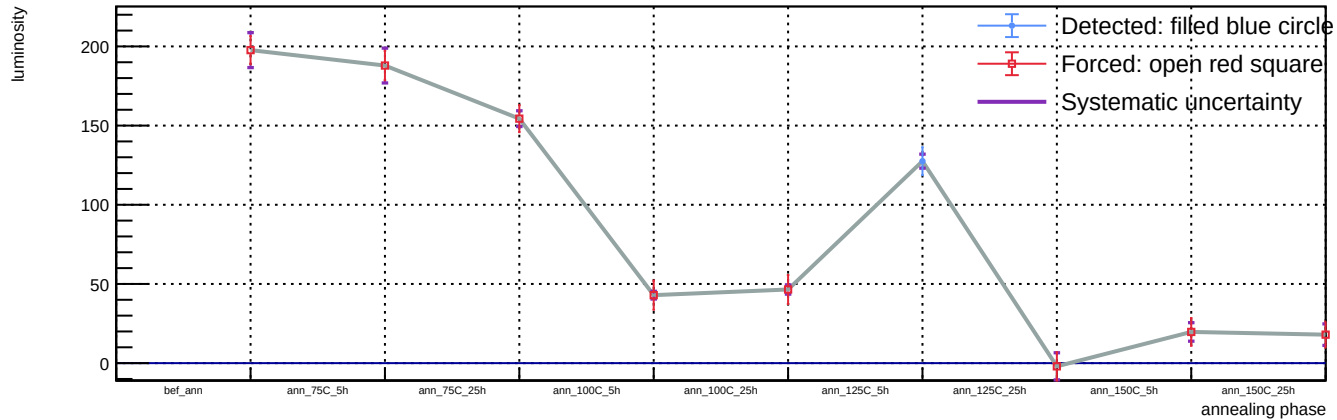
Sensor B1, T = 20\text{ C} , v_{\text{over}} = 5\text{ V} - Spot 96: luminosity vs phase
