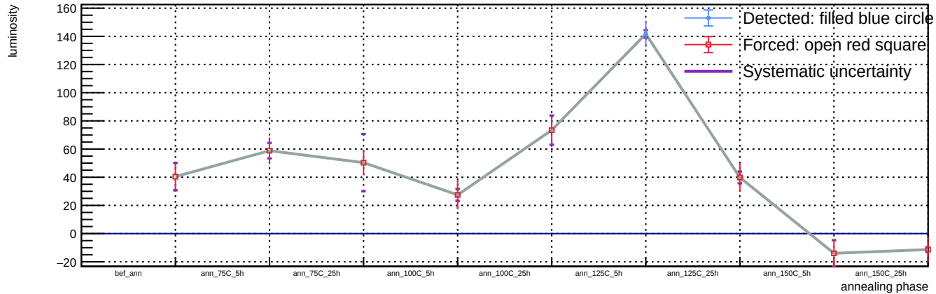
Sensor B1, T = 20\text{ C} , v_{\text{over}} = 5\text{ V} - Spot 97: luminosity vs phase
