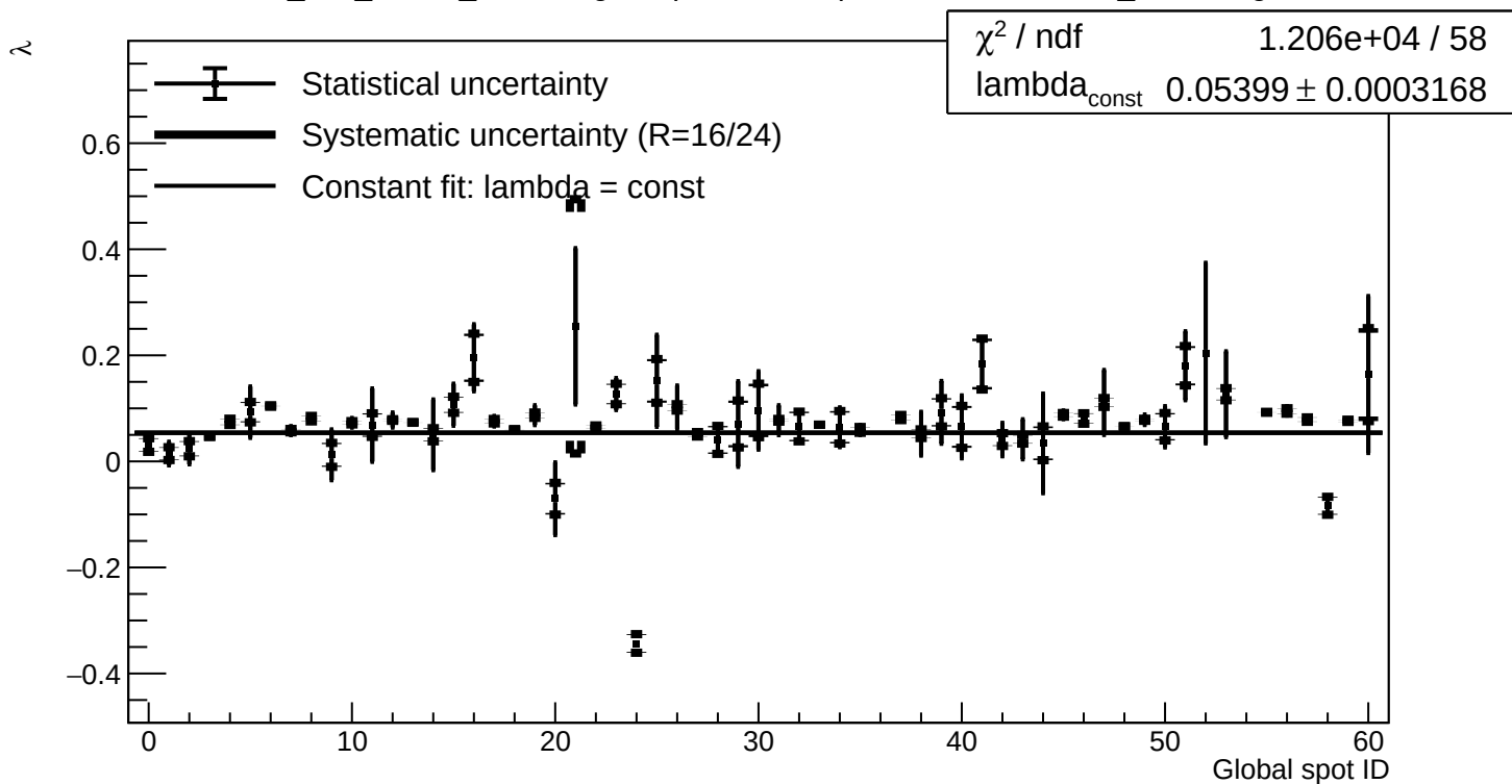
A1_v=5_before_annealing - Exponential fit parameter \lambda - before_annealing
