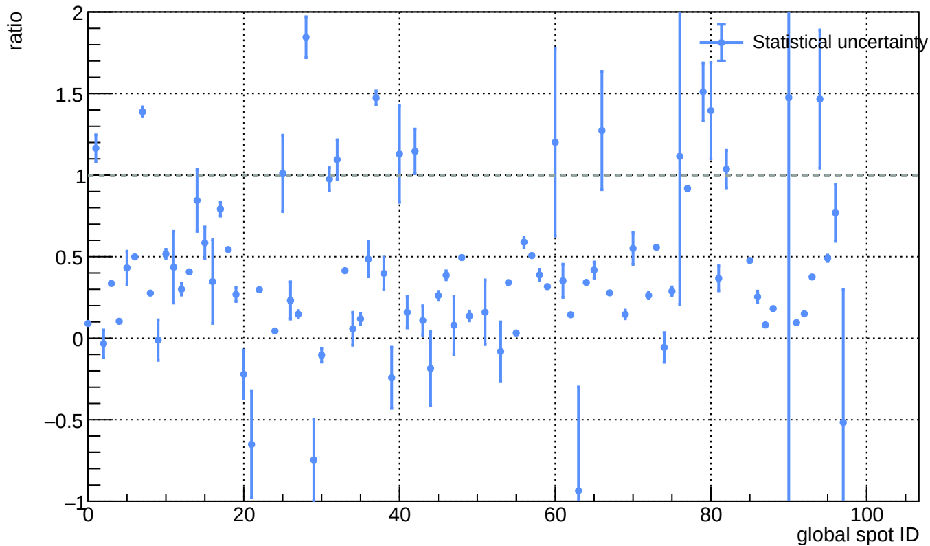
Sensor A1, T = 20\text{ C} - L(\text{ann\_125C\_5h}) / L(\text{before\_annealing})
