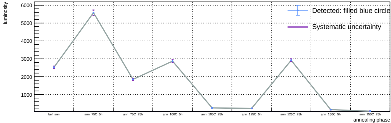
Sensor A1, T = 20 C, representative v = 58.3 V (max available) - Spot 0: luminosity vs phase
