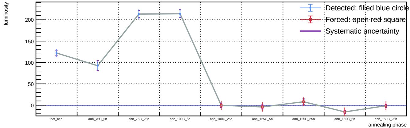
Sensor A1, T = 20 C, representative v = 58.3 V (max available) - Spot 2: luminosity vs phase
