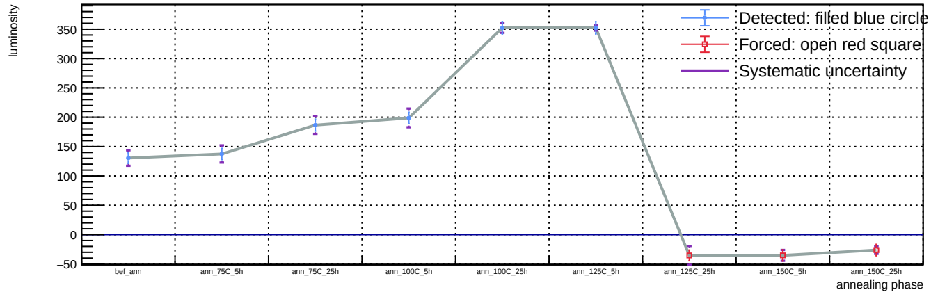
Sensor A1, T = 20 C, representative v = 58.3 V (max available) - Spot 23: luminosity vs phase
