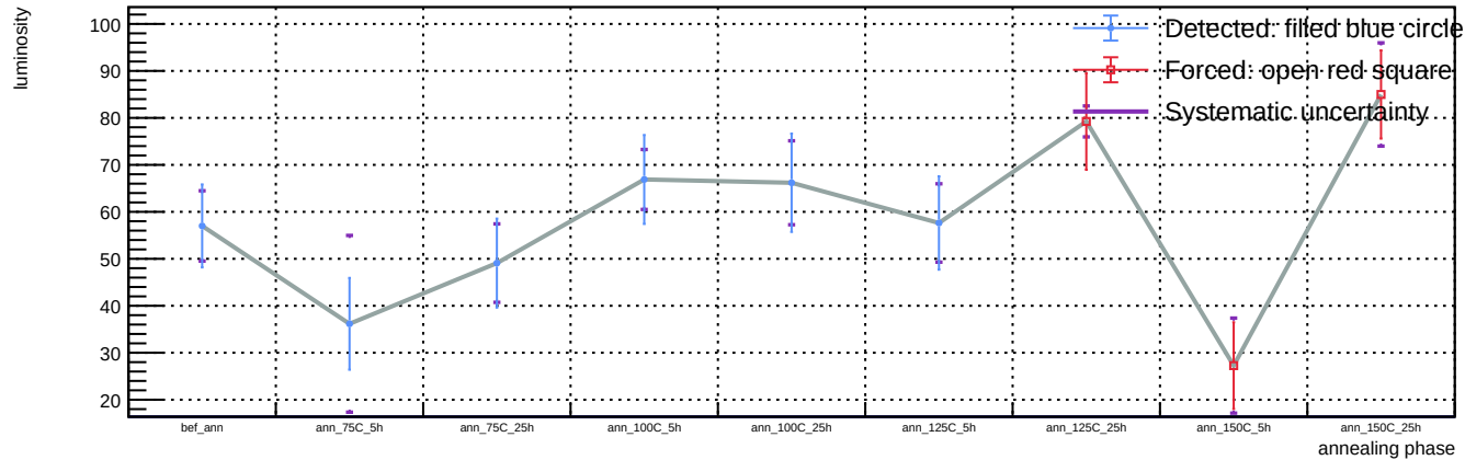
Sensor A1, T = 20 C, representative v = 58.3 V (max available) - Spot 25: luminosity vs phase
