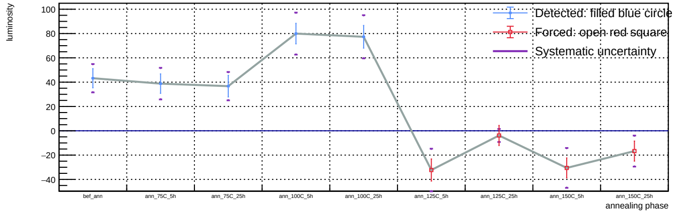
Sensor A1, T = 20 C, representative v = 58.3 V (max available) - Spot 29: luminosity vs phase
