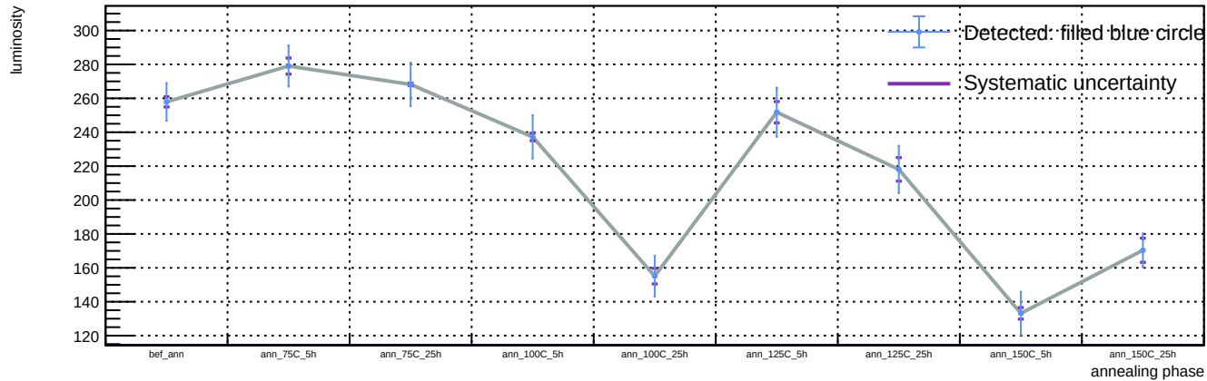
Sensor A1, T = 20 C, representative v = 58.3 V (max available) - Spot 31: luminosity vs phase
