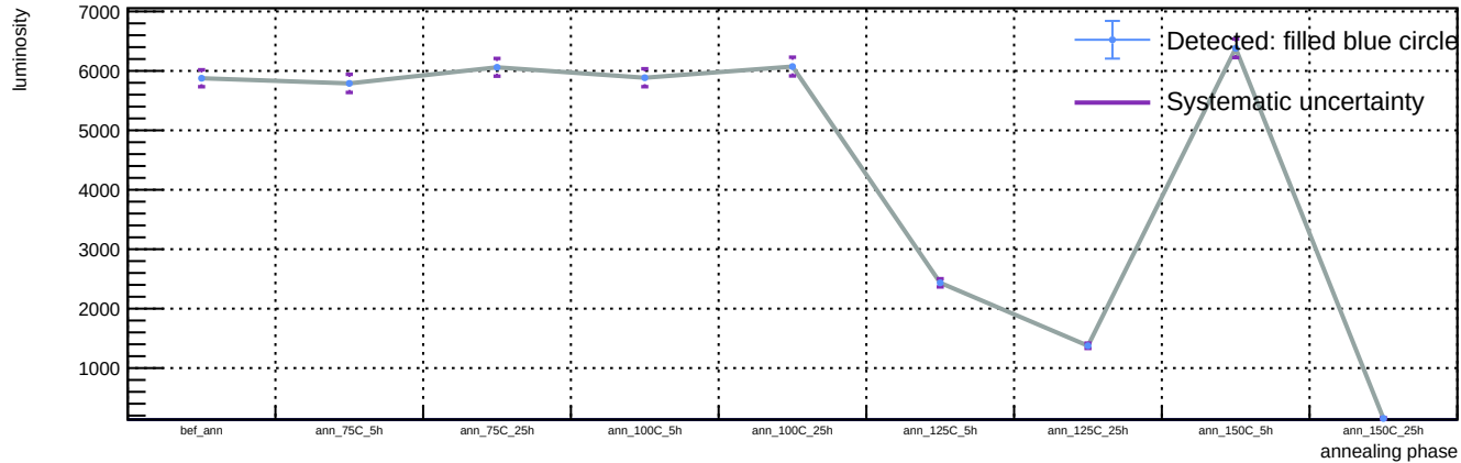
Sensor A1, T = 20 C, representative v = 58.3 V (max available) - Spot 33: luminosity vs phase
