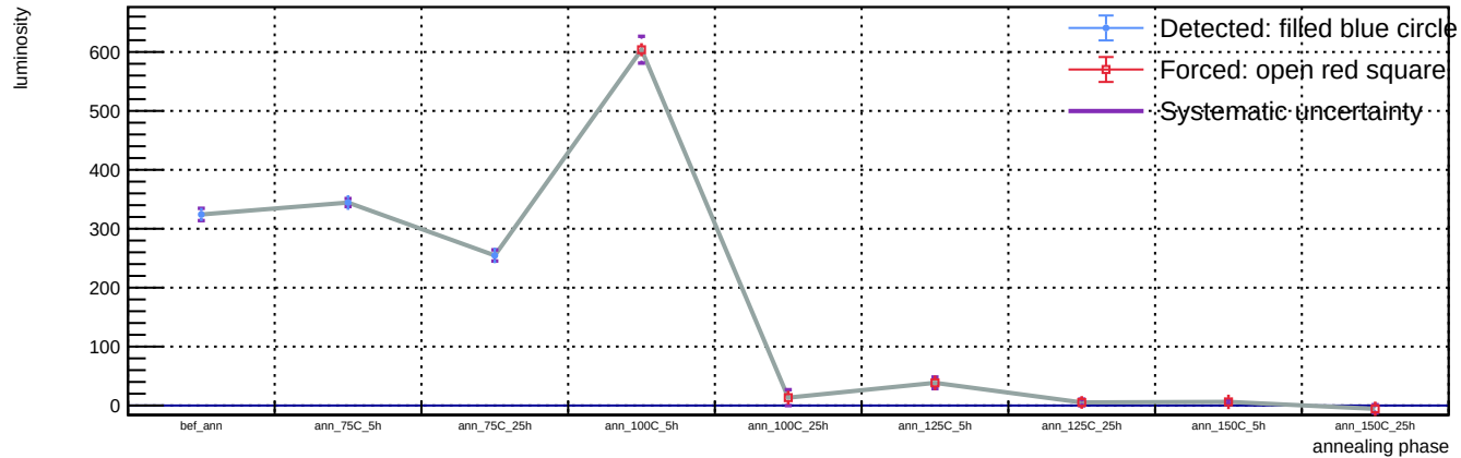
Sensor A1, T = 20 C, representative v = 58.3 V (max available) - Spot 35: luminosity vs phase
