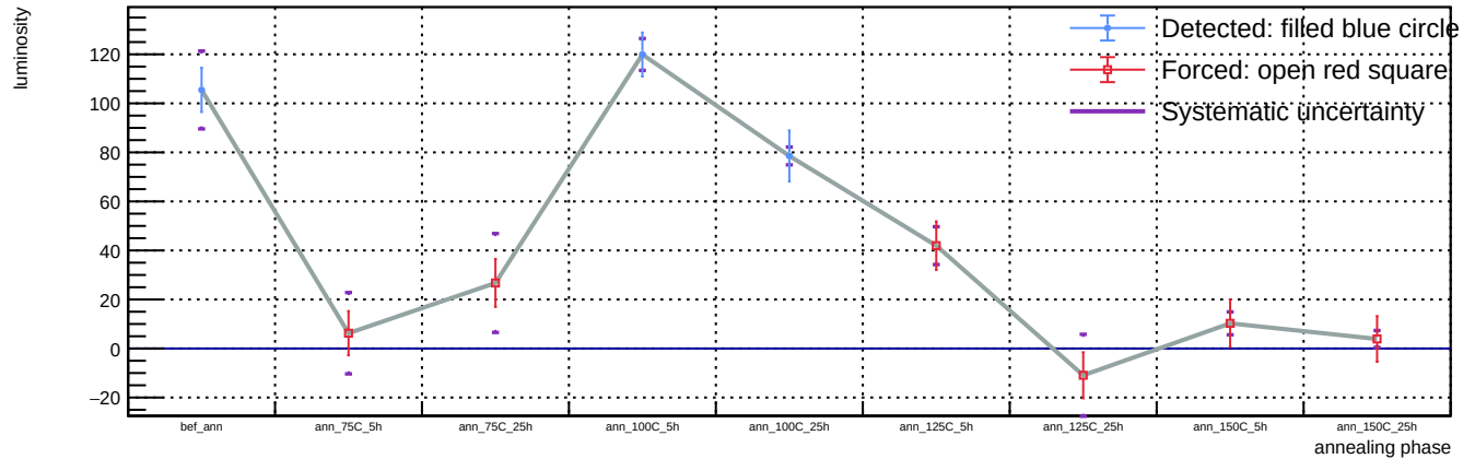
Sensor A1, T = 20 C, representative v = 58.3 V (max available) - Spot 38: luminosity vs phase
