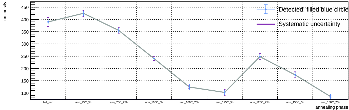
Sensor A1, T = 20 C, representative v = 58.3 V (max available) - Spot 45: luminosity vs phase
