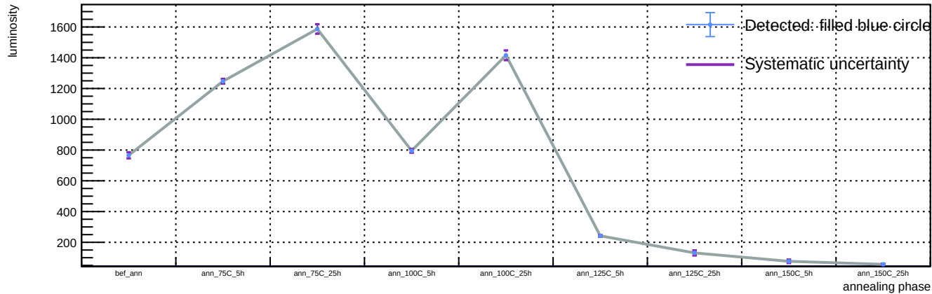
Sensor A1, T = 20 C, representative v = 58.3 V (max available) - Spot 59: luminosity vs phase
