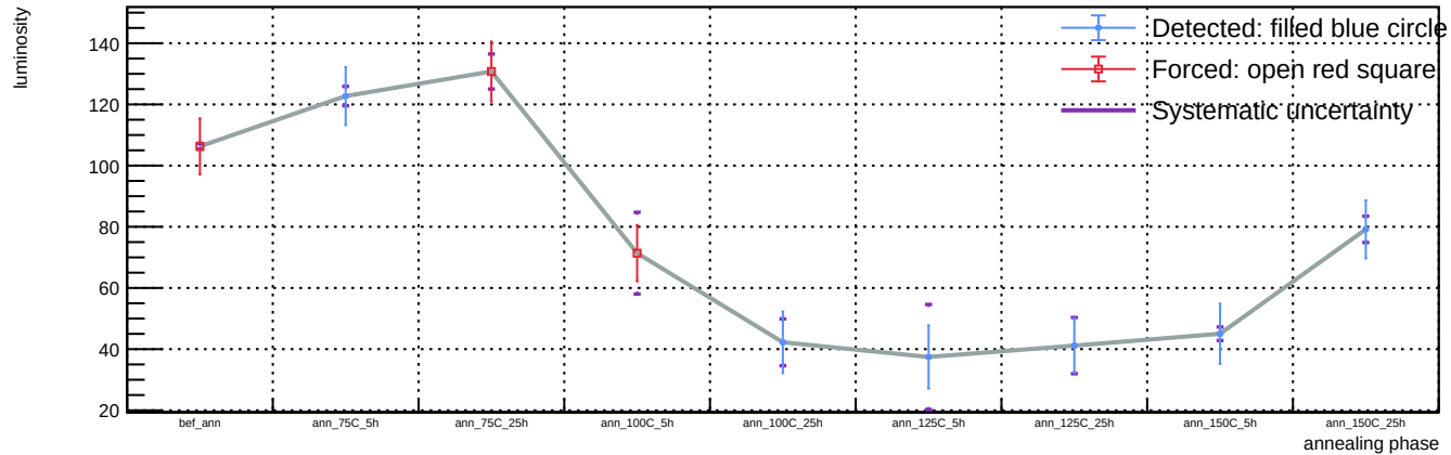
Sensor A1, T = 20 C, representative v = 58.3 V (max available) - Spot 61: luminosity vs phase
