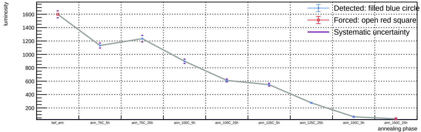
Sensor A1, T = 20 C, representative v = 58.3 V (max available) - Spot 64: luminosity vs phase
