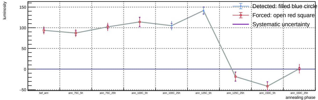
Sensor A1, T = 20 C, representative v = 58.3 V (max available) - Spot 79: luminosity vs phase
