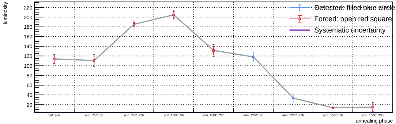
Sensor A1, T = 20 C, representative v = 58.3 V (max available) - Spot 82: luminosity vs phase
