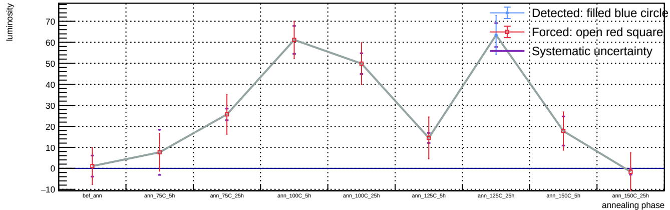
Sensor A1, T = 20 C, representative v = 58.3 V (max available) - Spot 84: luminosity vs phase
