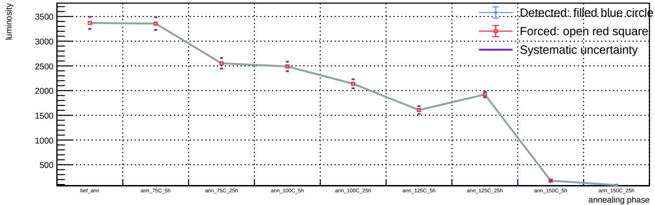
Sensor A1, T = 20 C, representative v = 58.3 V (max available) - Spot 85: luminosity vs phase
