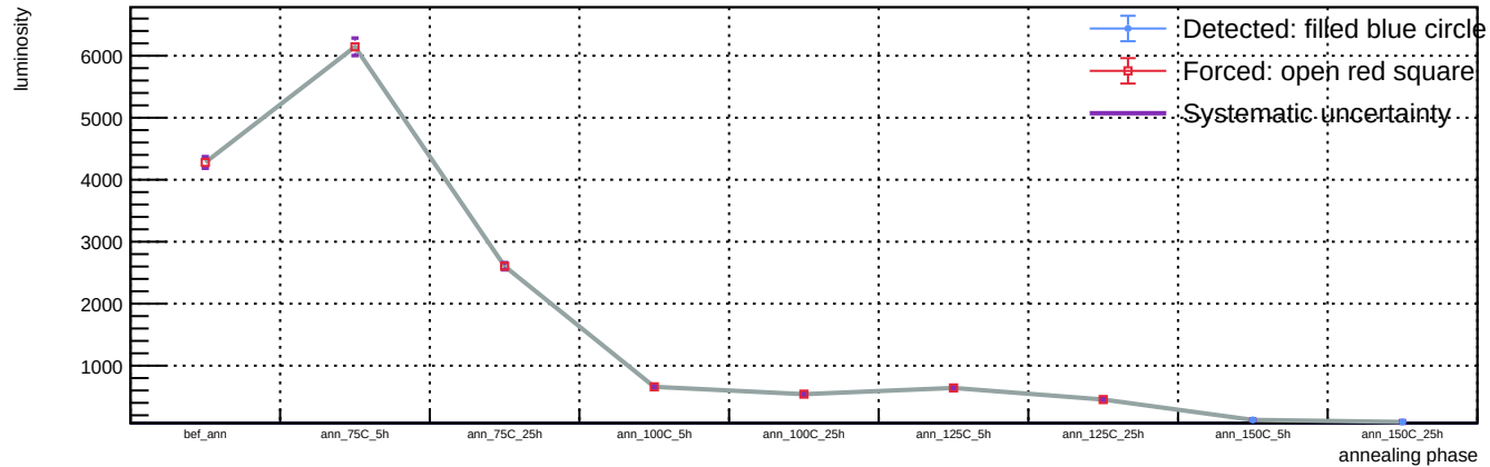
Sensor A1, T = 20 C, representative v = 58.3 V (max available) - Spot 92: luminosity vs phase
