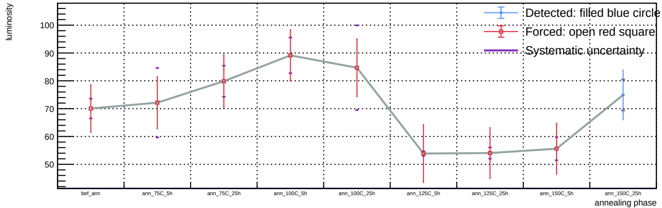
Sensor A1, T = 20 C, representative v = 58.3 V (max available) - Spot 96: luminosity vs phase
