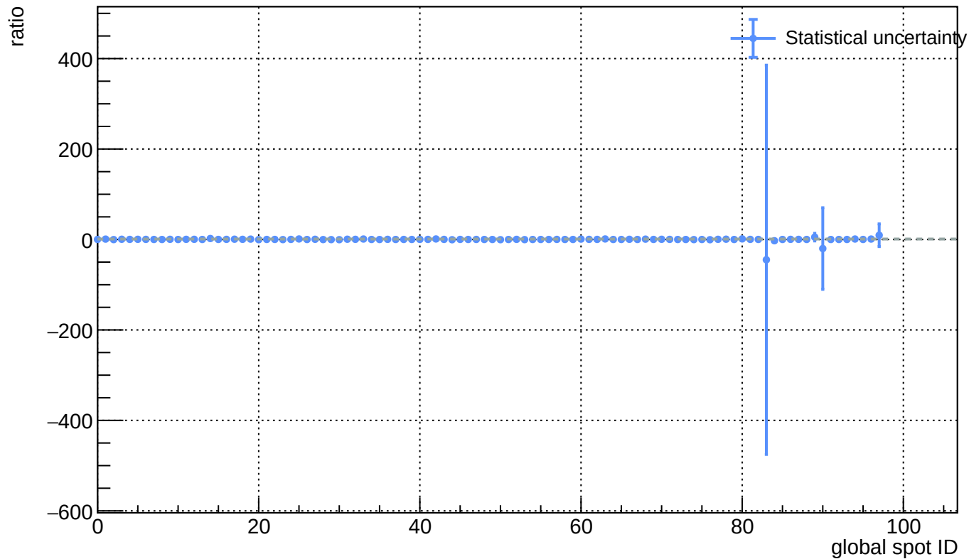
Sensor A1, v = 5 \text{ V} - L(\text{ann\_150C\_5h}) / L(\text{before\_annealing})
