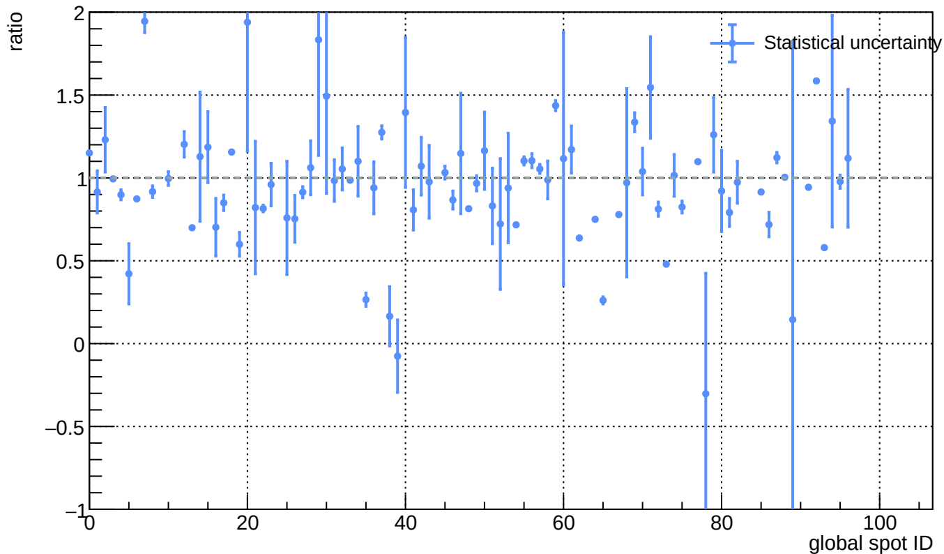
Sensor A1, v = 5\text{ V} - L(\text{ann\_75C\_5h}) / L(\text{before\_annealing})
