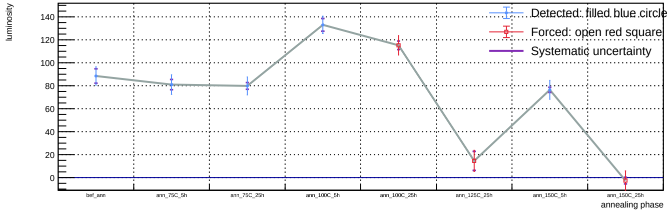
Sensor A1, v = 5 V, representative T = 23 C (max available) - Spot 1: luminosity vs phase
