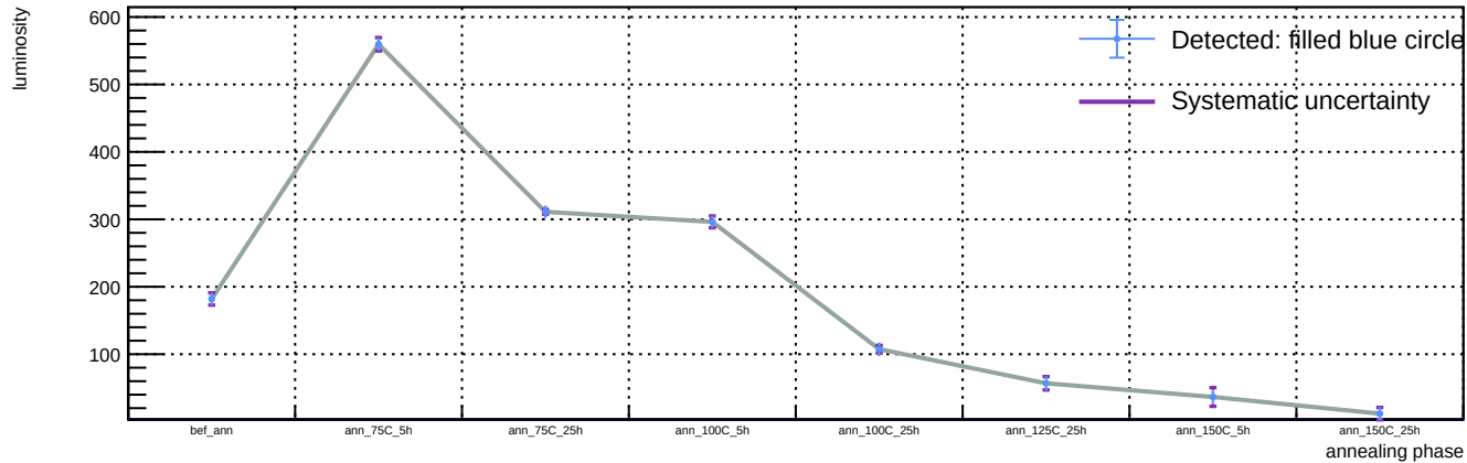
Sensor A1, v = 5 V, representative T = 23 C (max available) - Spot 24: luminosity vs phase
