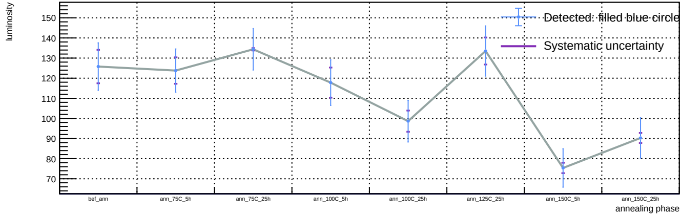
Sensor A1, v = 5 V, representative T = 23 C (max available) - Spot 31: luminosity vs phase
