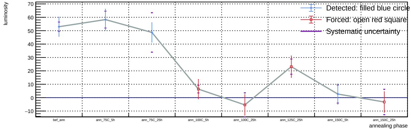
Sensor A1, v = 5 V, representative T = 23 C (max available) - Spot 34: luminosity vs phase
