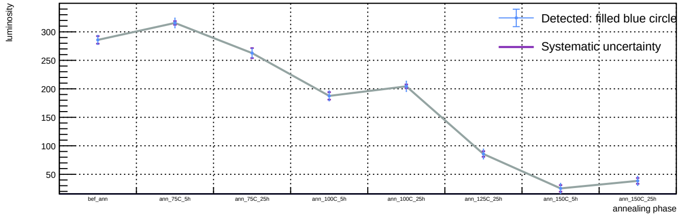
Sensor A1, v = 5 V, representative T = 23 C (max available) - Spot 56: luminosity vs phase
