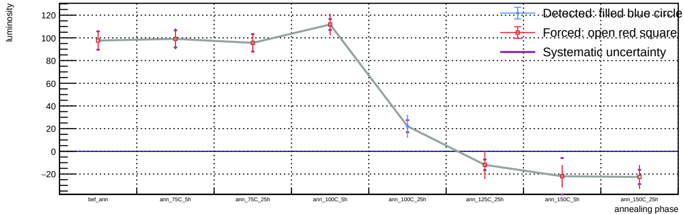
Sensor A1, v = 5 V, representative T = 23 C (max available) - Spot 74: luminosity vs phase
